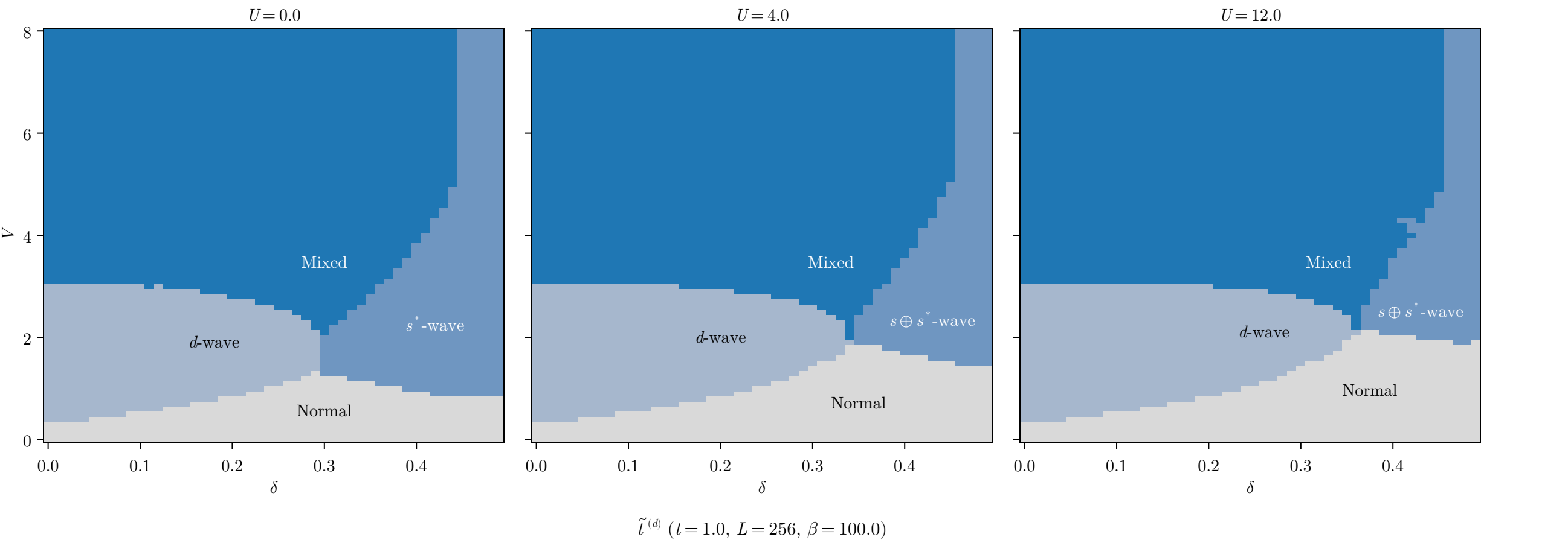
SC and normal regions ( t = 1.0, L = 256, \beta = 100.0 )
